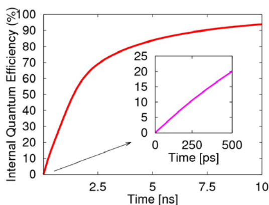
Figure 7. Evolution of the electroluminescent internal quantum efficiency, including the decay of the singlet exciton and emission from the two-transition process of the triplet exciton.
