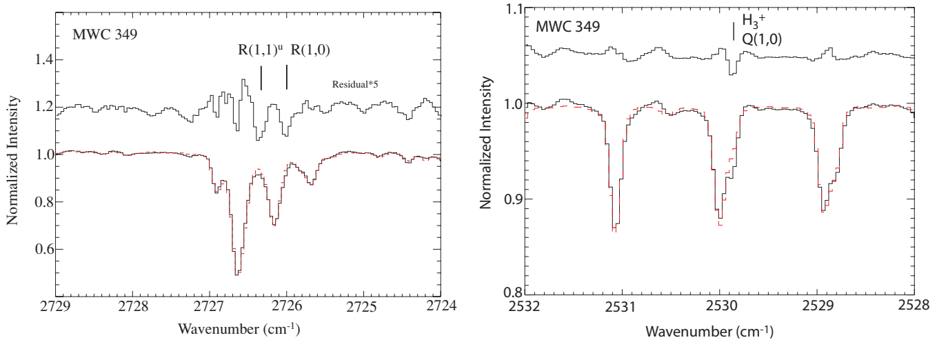
Figure 4. Normalized L -band spectra of MWC 349 (solid line) showing the detection of the R(1,1)^u and R(1,0) , and Q(1,0) lines of \text{H}_3^+ . The telluric model is overlotted (dashed line). Plotted above is the residual, displaced vertically for clarity.
